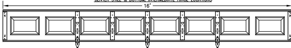
CENTER STILE & BOTTOM, INTERMEDIATE HINGE LOCATIONS
